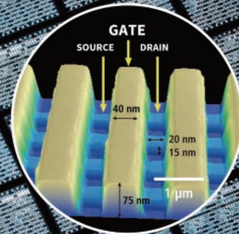
AFM image of 3D FinFET Structure
